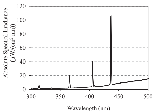
Fig. 1 Absolute irradiance of the sun lamp
