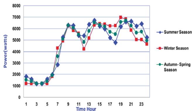
Fig. 1 Daily load curve for six families
