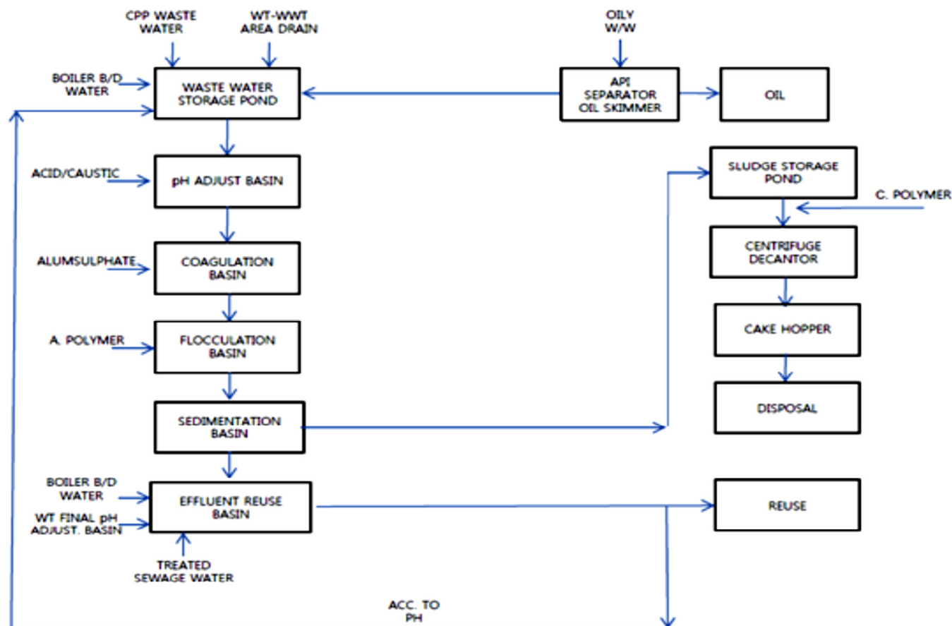
Fig. 2 WWTP Flow Diagram
