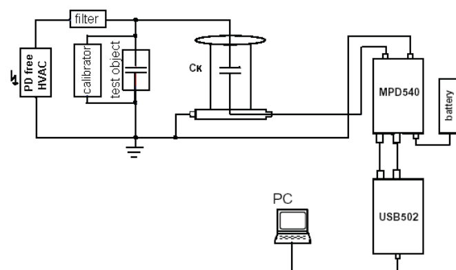
Fig. 4 Circuit connection
