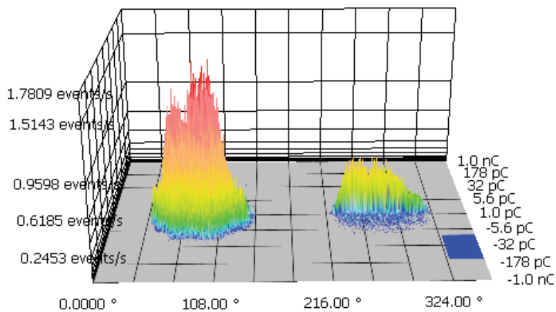
Fig. 6 3D PD Histogram of a clean duct at 0.1 MPa
