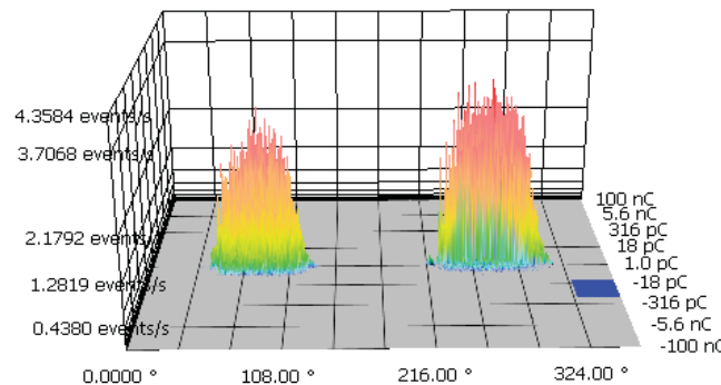
Fig. 12 3D PD Histogram with copper particle at 0.1 MPa
