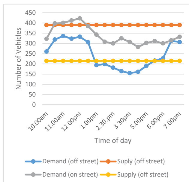
Fig. 3 Parking demand & supply in Week day
