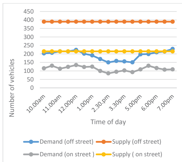
Fig. 2 Parking demand & supply in Weekend day
