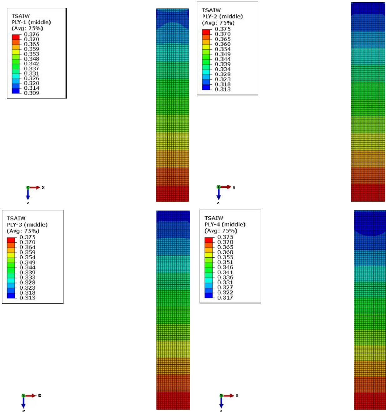
Fig. 6 Case B failure index (4 Plies)
