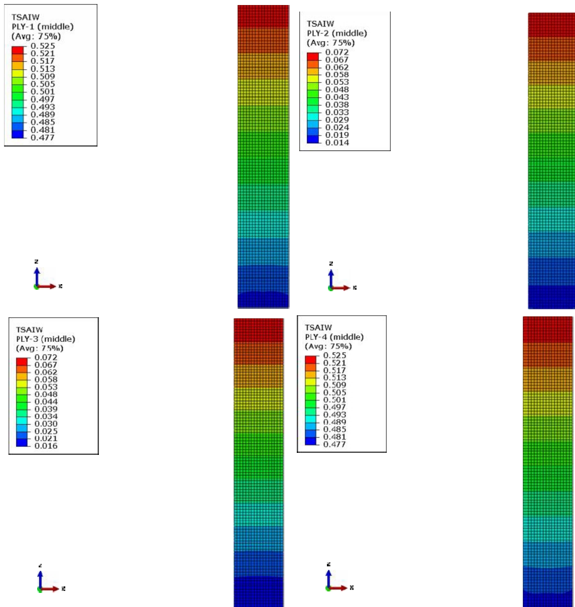
Fig. 7 Case C failure index (4 Plies)
