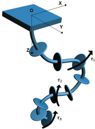
Fig. 1 Flexible technological arm
