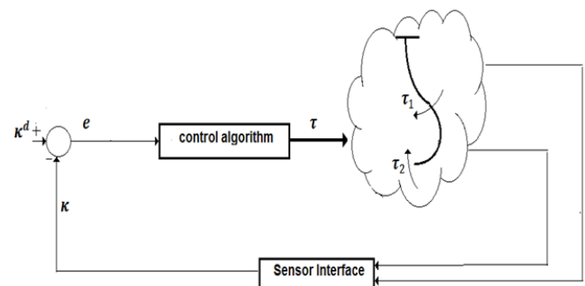
Fig. 4 Manipulator control system
