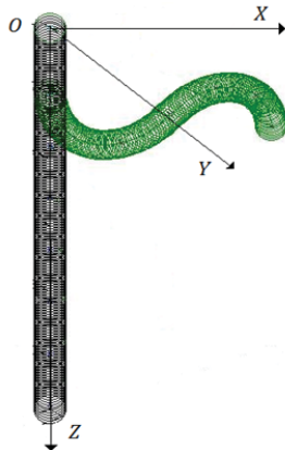
Fig. 6 3D motion \kappa_{10d} = -\frac{\pi}{14}, \kappa_{1qd} = -\frac{\pi}{64}, \kappa_{20d} = \frac{\pi}{14}, \kappa_{2qd} = -\frac{\pi}{64}
