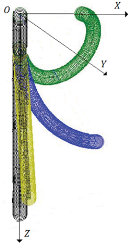
Fig. 5 3D motion: \kappa_{10d} = \kappa_{20d} = -\frac{\pi}{14}, \kappa_{1qd} = \kappa_{2qd} = -\frac{\pi}{64}
