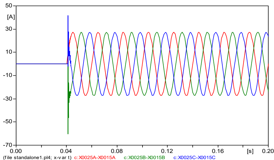
Fig. 15 Using pre-insertion resistor to mitigate the transient
