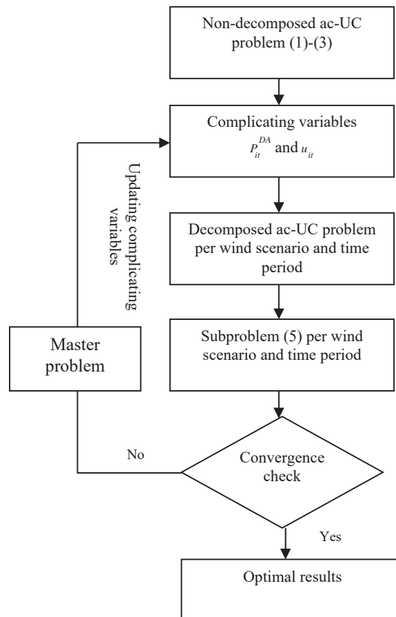
Fig. 1 Flowchart for Bender's Algorithm
