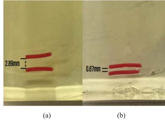
Fig. 3 The wire phantom spaced (a) 2.89mm (b)0.87mm
