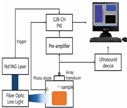
Fig. 2 Real-time photoacoustic system block diagram
