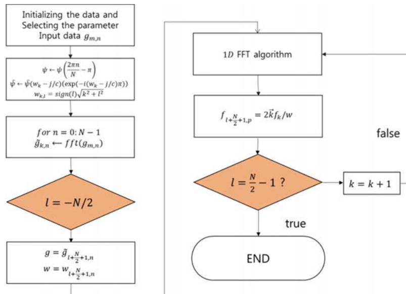
Fig. 1 Flow chart of 2D non-uniform FFT algorithm
