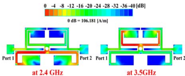
Fig. 5 Current distribution of the proposed filter
