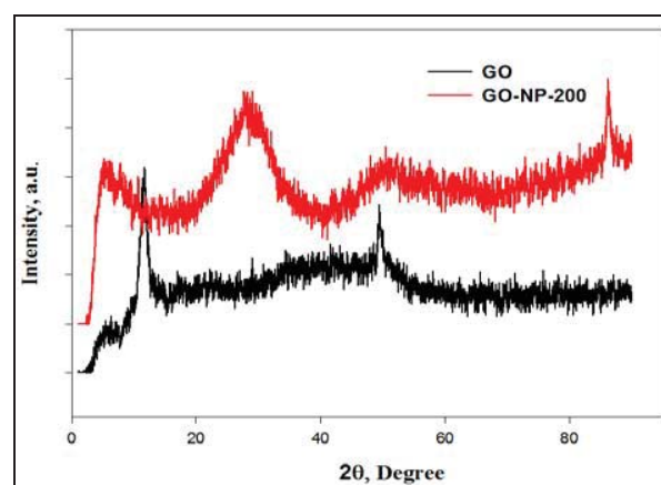
Fig. 1 XRD patterns of GO and GO-NP-200
