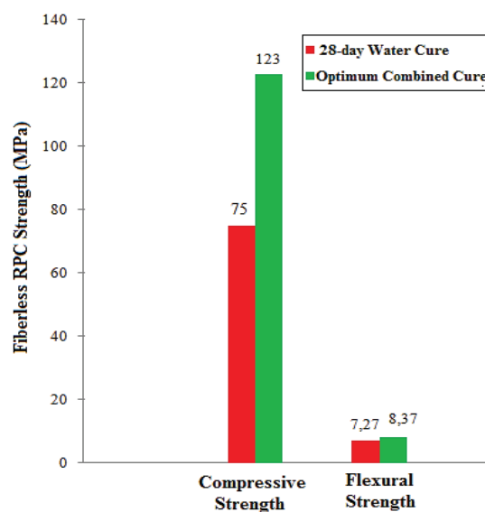
Fig. 2 Compressive and Flexural Strength of Fiberless RPC
