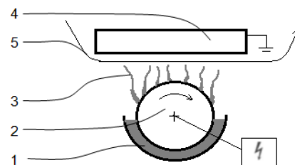
Fig. 4 Nanospider™ machine: (1) polymer or melt liquid, (2) cylinder, high-voltage source, (3) emerging nanofibers, (4) grounded collector, catching nanofibers, (5) supportlayer for nanofibers [4]
