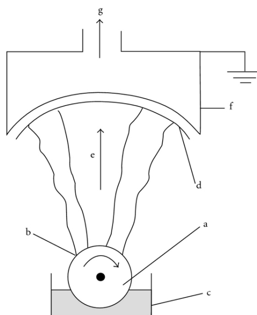
Fig. 1 Nanospider™ equipment for production of nanofibers by electrostatic spinning: (a) electrode metal roller as positive electrode, (b) fiberforming polymer layer, (c) reservoir of polymer solution, (d) textile substrate (supportive material), (e) fiber formation direction, (f) electrode earthing shield, (g) air suction [10]
