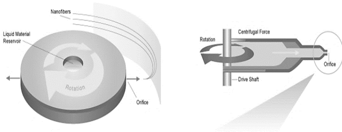
Fig. 5 Forcespinning process [19]
