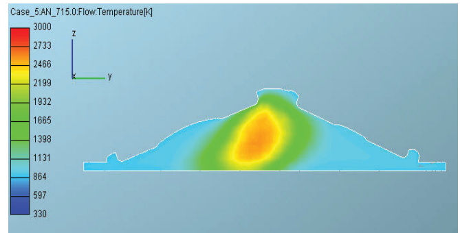
Fig. 4 Spatial distribution of temperature in y-z plane, x=const. at 355 deg. ATDC, k- \epsilon , CH 4
