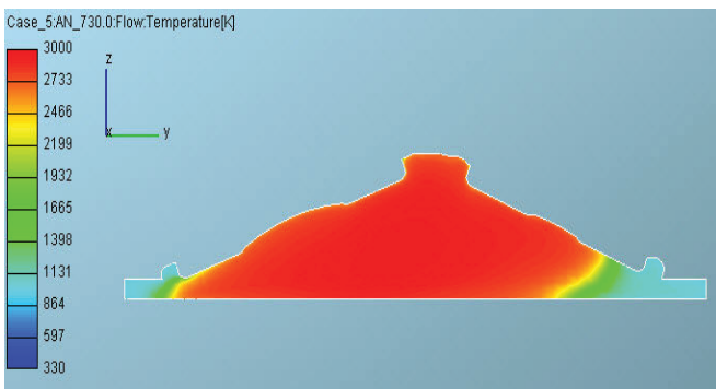
Fig. 10 Spatial distribution of temperature in y-z plane, x=\text{const.} at 370 deg. ATDC, k-\epsilon , CH4
