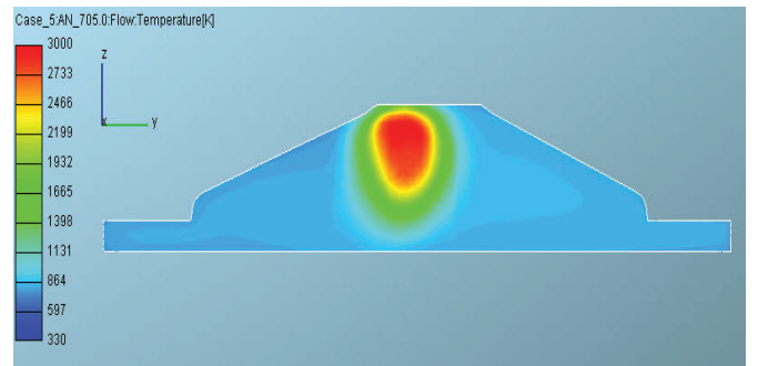
Fig. 12 Spatial distribution of temperature in y-z symmetry plane, x=0.0 at 345 deg. ATDC, k-\epsilon , CH4
