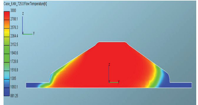
Fig. 19 Spatial distribution of temperature in y-z symmetry plane, x=0.0 at 365 deg. ATDC, k- \epsilon , C8H18
