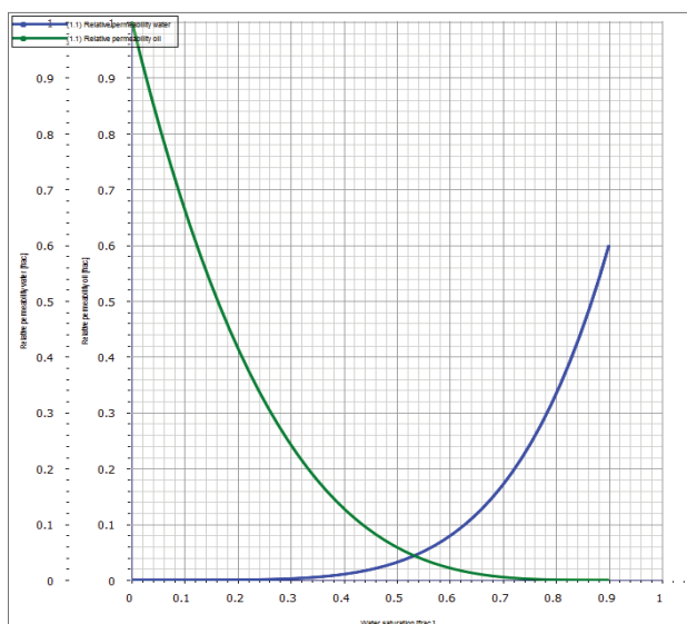
Fig. 3 Relative permeability ( K_r ) estimation using Corey / Skjaveland correlation
