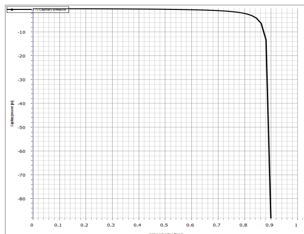
Fig. 5 Capillary Pressure ( P_c ) estimation using Corey / Skjaveland correlation
