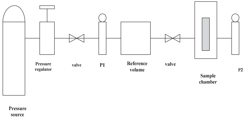
Fig. 1 Schematics of a Boyle's law porosimeter
