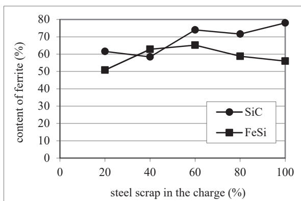
(a) Content of ferrite in the matrix
