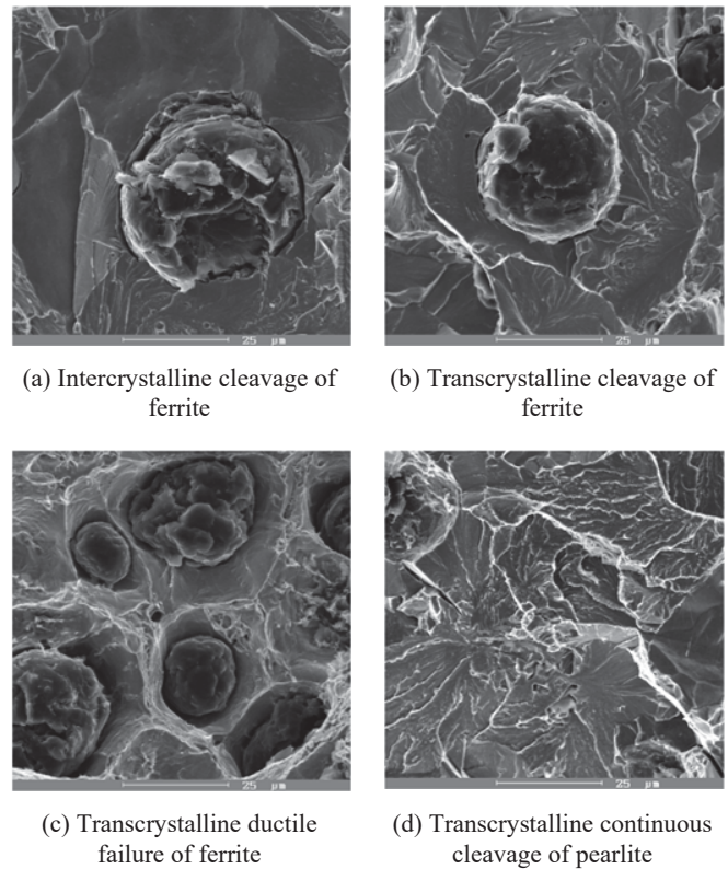
Fig. 6 Failure micro mechanisms at static stress, SEM
