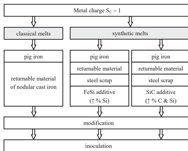
Fig. 1 Scheme of the production of nodular cast iron
