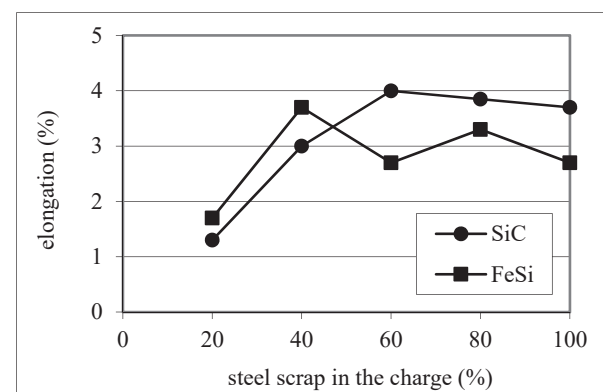
(b) Elongation
