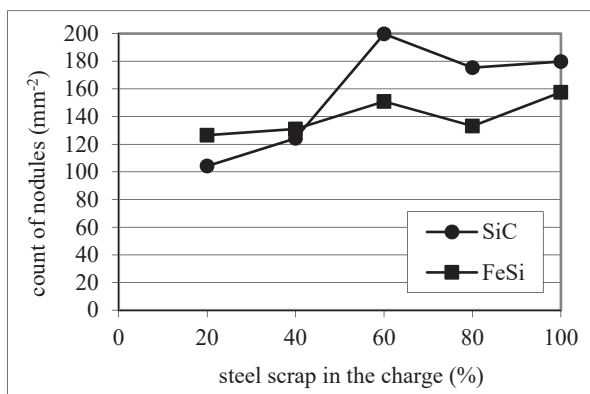
(b) Count of graphitic nodules
