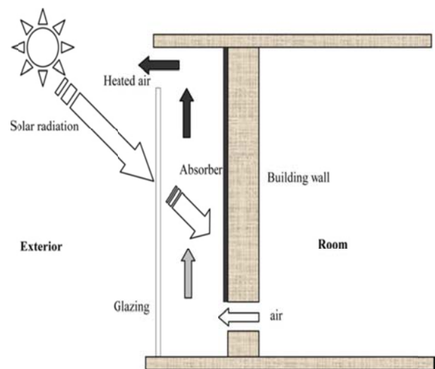
Fig. 3 Schematic diagram of solar chimney [30]
