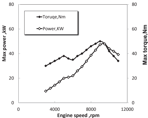
Fig. 3 Output power and torque in rear wheels of NA engine
