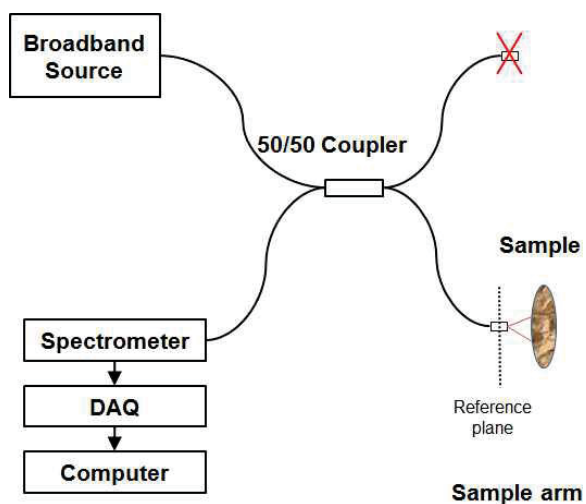
Fig. 1 Block diagram of the CP-FD-OCT system
