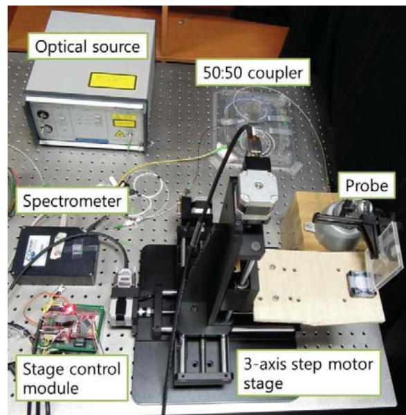
Fig. 2 Photograph of the CP-FD-OCT system
