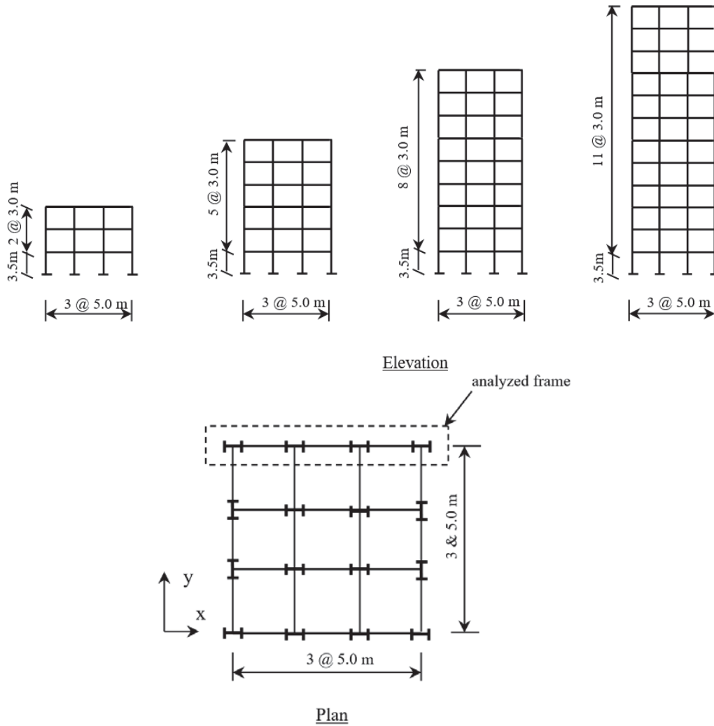
Fig. 2 Schematic representation of the frames
