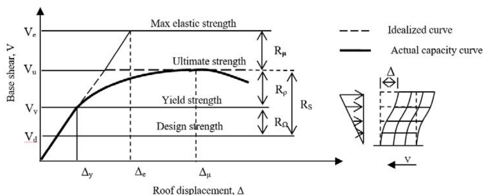
Fig. 1 Relationship between base shear and roof displacement
