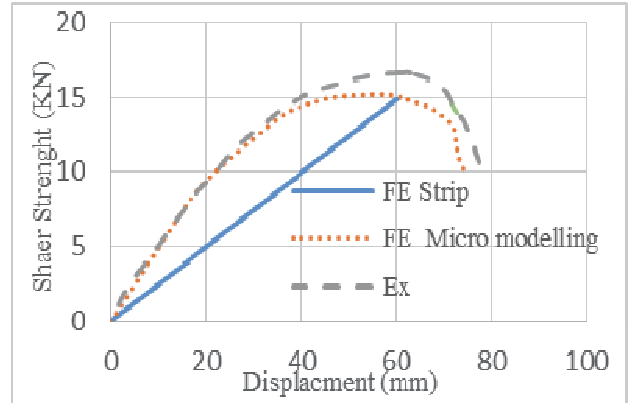
Fig. 7 Shear-displacement curve of SWP-CFS under control displacement
