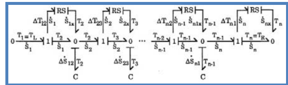
Fig. 3 Modified heat conduction BG [1]
