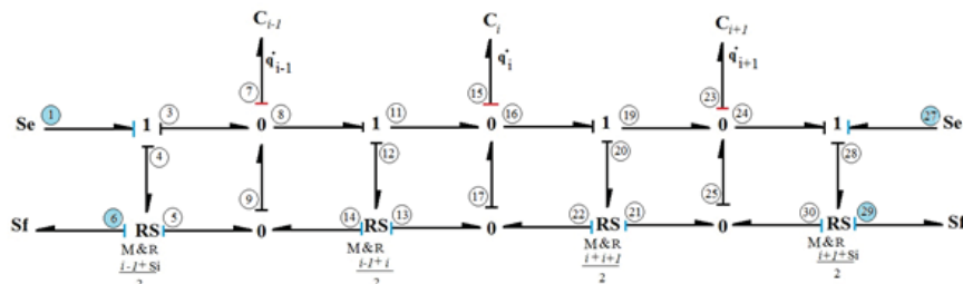
Fig. 5 1D conduction BG model
