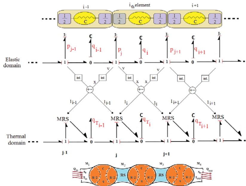
Fig. 6 Geometrical connectivity of thermal and elastic domains
