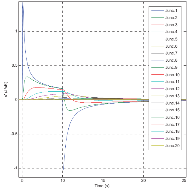
Fig. 9. Junction entropy flows
