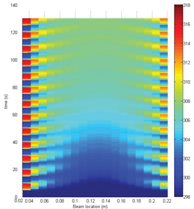
Fig. 12 Temperature contour alongside the beam during the periodic thermal pulse input from both ends
