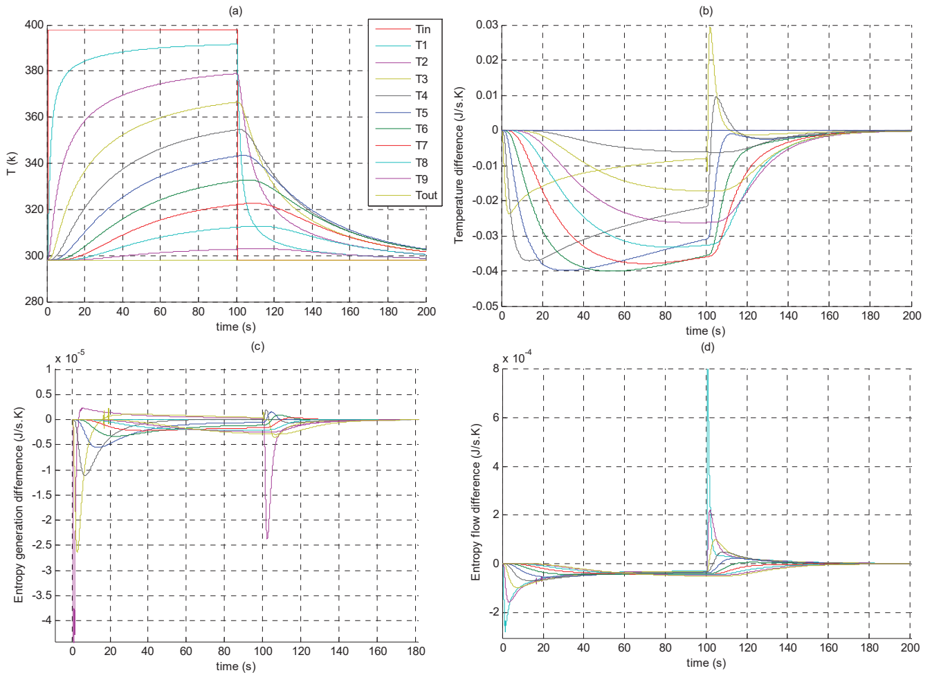
Fig. 14 Expansion impact on system conductivity: (a) Element temperature change due to pulse input at left side; (b) Difference in thermal behavior between fixed and expansive geometry situations; (c) Difference in entropy generation; (d) Difference in reversible entropy flow
