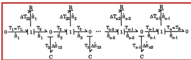
Fig. 1 Conventional BG heat conduction model [3]
