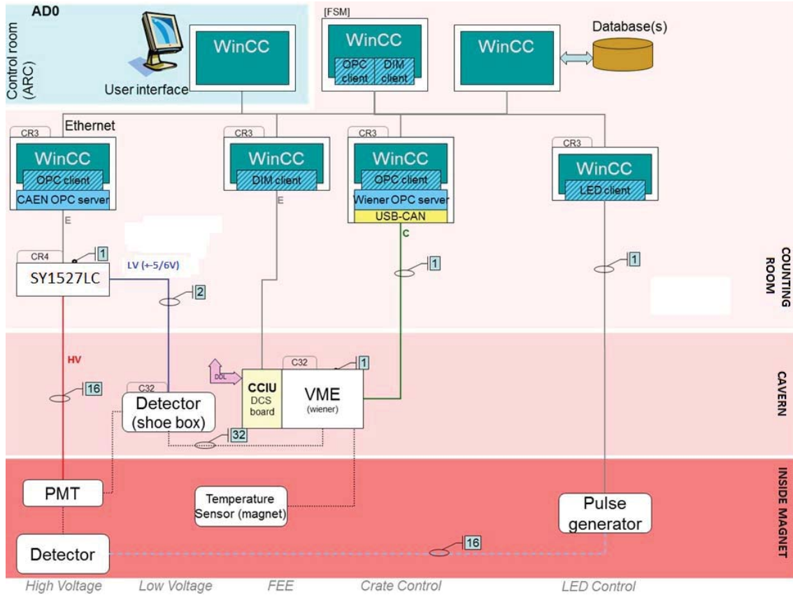
Fig. 3 Hardware architecture of AD0 DCS
