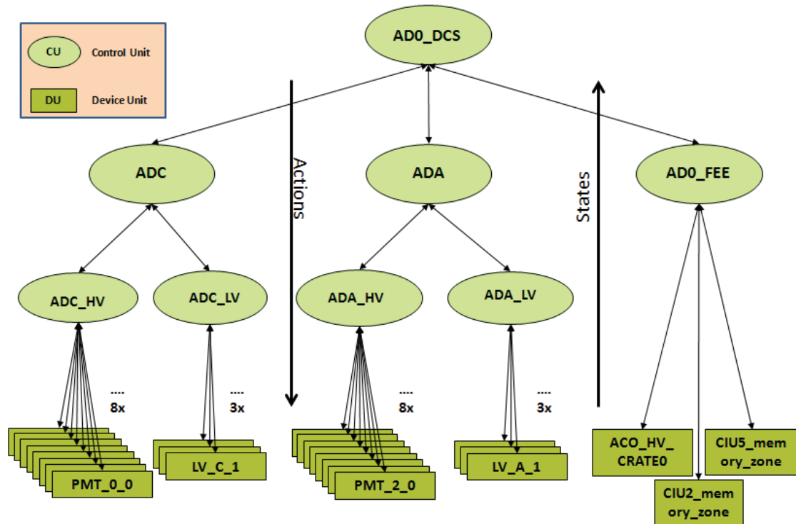
Fig. 4 AD0 DCS Software Architecture
