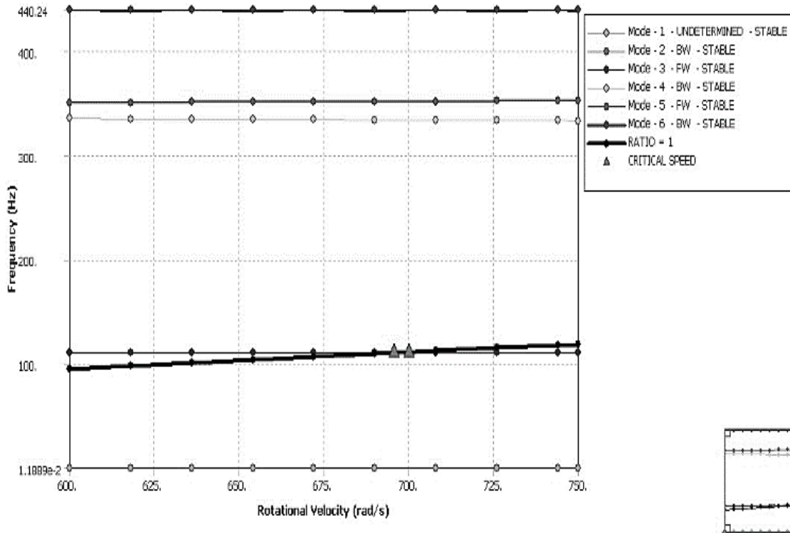
Fig. 12 Campbell diagram
