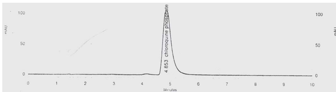
Fig. 4 HPLC Chromatogram
