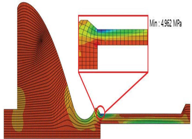
Fig. 8 Maximum tensile stress of weir structure, using the IFE model
