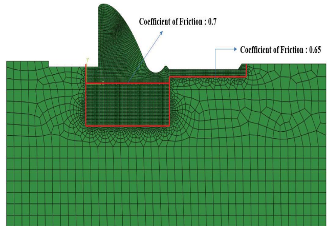
Fig. 4 FE model with friction elements
