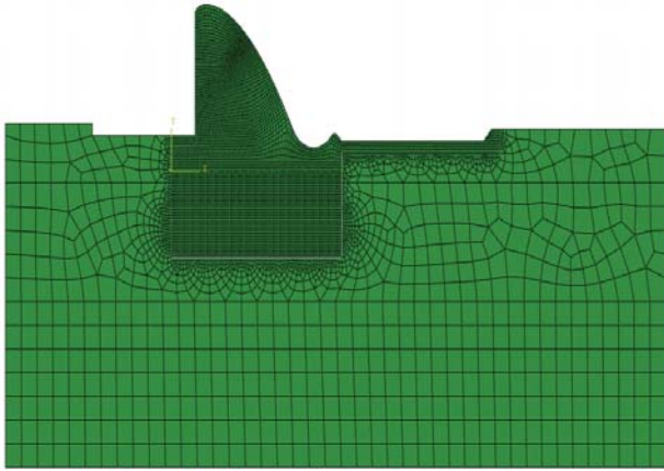
Fig. 1 FE model of weir structure
