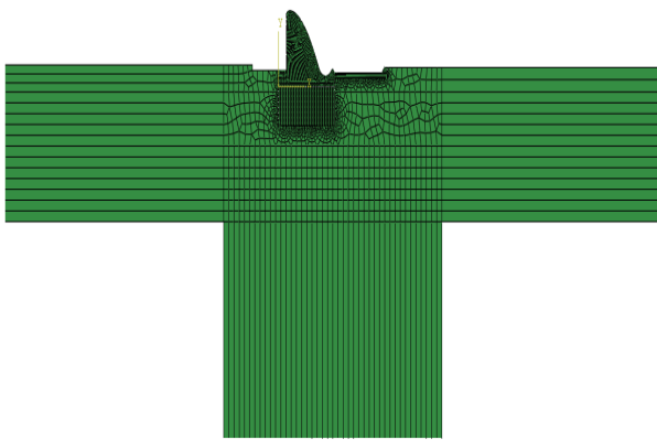
Fig. 2 IFE model of weir structure
