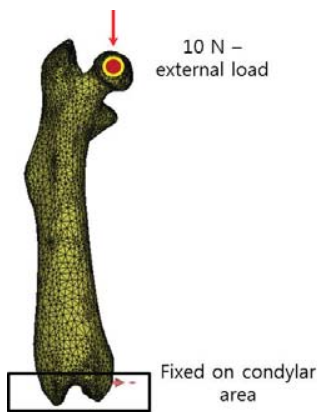
Fig. 3 Boundary conditions for finite element analysis
