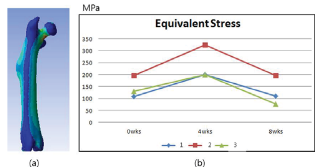
Fig. 7 (a) Result of finite element analysis for equivalent stress (b) Equivalent stress at 4 and 8 weeks after ovariectomy compared to 0 week in each specimen
