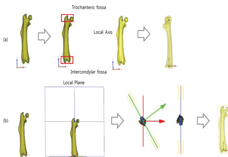
Fig. 2 The schematic illustrations of the re-arrangement of a femur for conducting finite element analysis (a) Aligned the local z-axis was aligned with the global Z-axis, (b) The local x-z plane was aligned with the global X-Z plane
