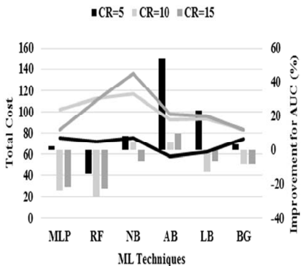
Fig. 4 Total Cost & AUC Improvement for Calendar using MetaCost
