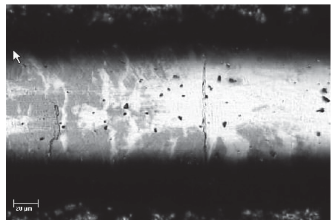
Fig. 2 Partial delamination of coating
