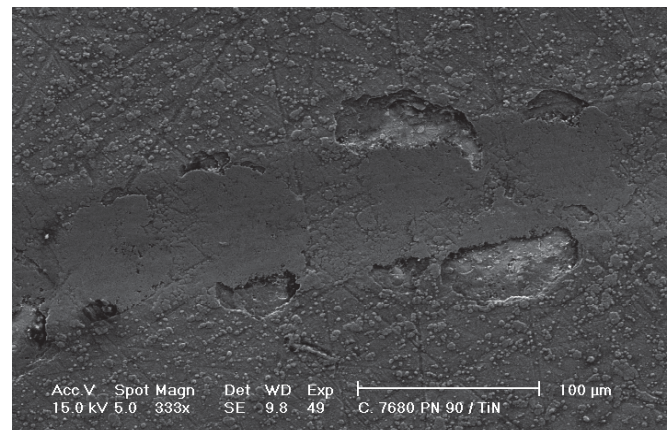
Fig. 3 SEM morphology of scratch test: pn/TiN(PVD)
