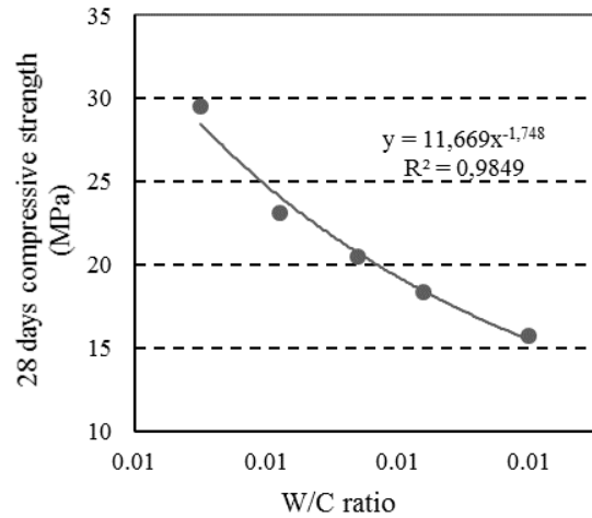
Fig. 3 Effect of W/C ratio on 28 day compressive strengths of the elaborated mortars
