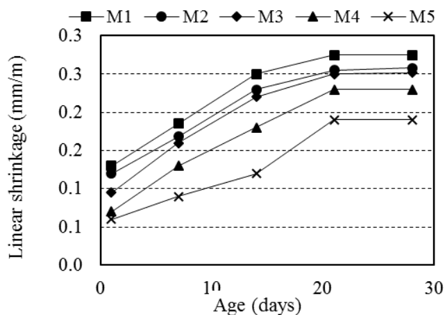
Fig. 4 Linear shrinkage of the elaborated mortars
