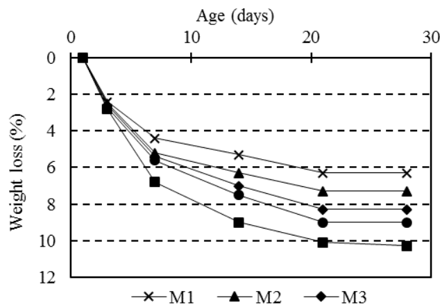
Fig. 5 Weight loss evolution of the elaborated mortars
