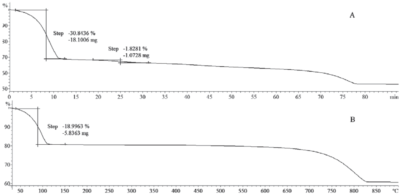
Fig. 1 TGA curves of sample SI3 (A) and SI4 (B)
