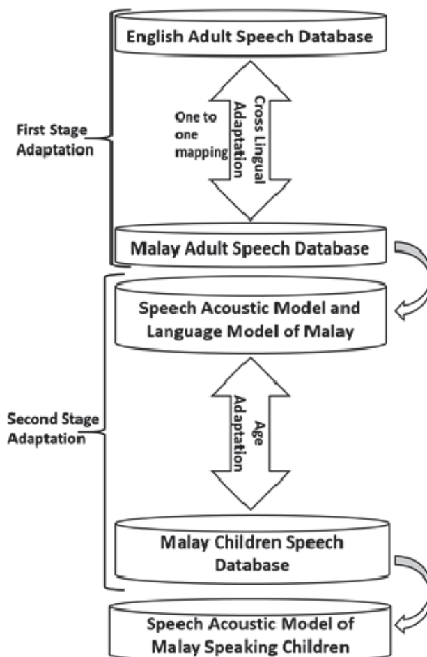
Fig. 1 The Framework of the Two Stage Adaptation for Developing ASR System for Malay Speaking Children
