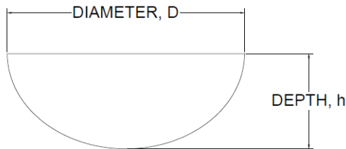
Fig. 5 Dimple ratio
