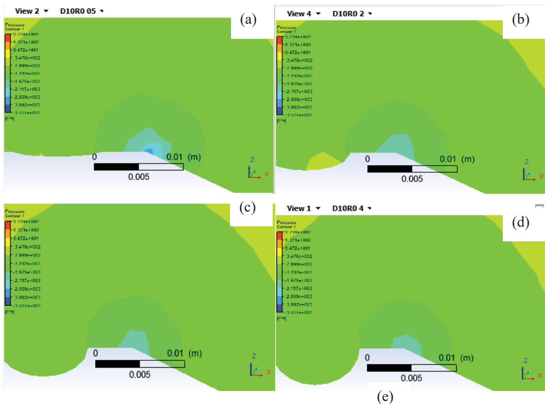
Fig. 6 Pressure contour for model with smooth surface
