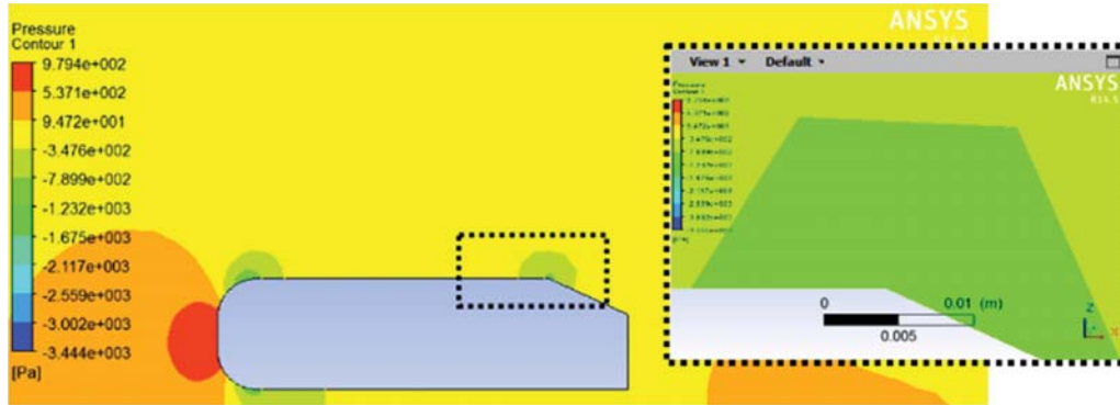
Fig. 6 Pressure contour for model with smooth surface
