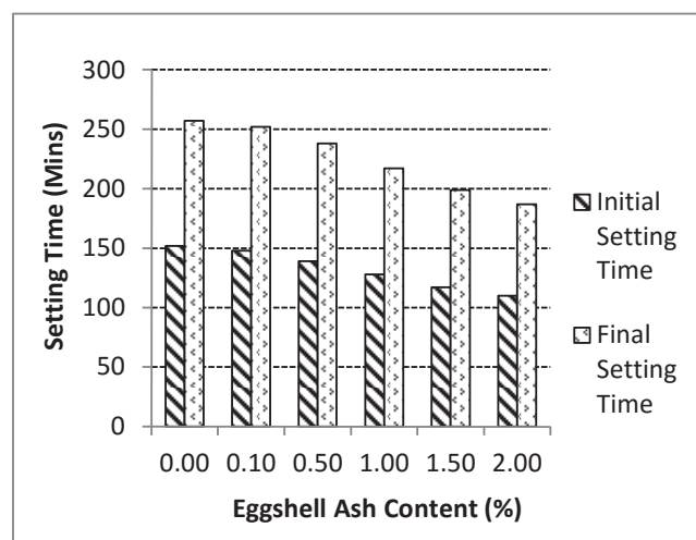
Fig. 5 Setting time vs Eggshells Ash
