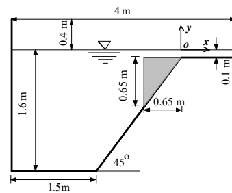
Fig. 1 Computational domain sand sliding into channel
