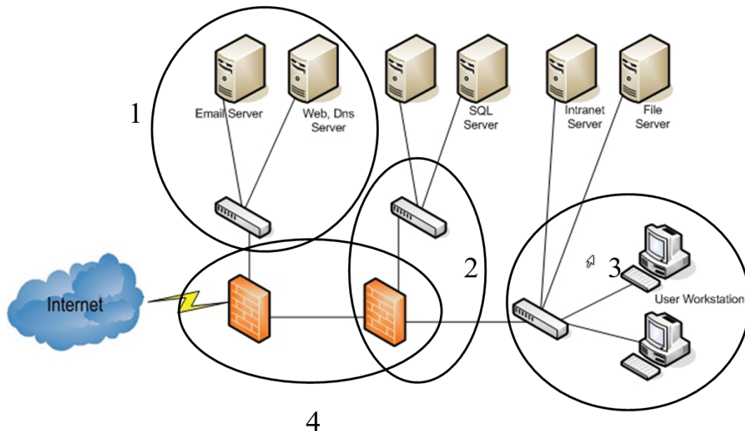
Fig. 2 Defense-in-Depth principle [5]
