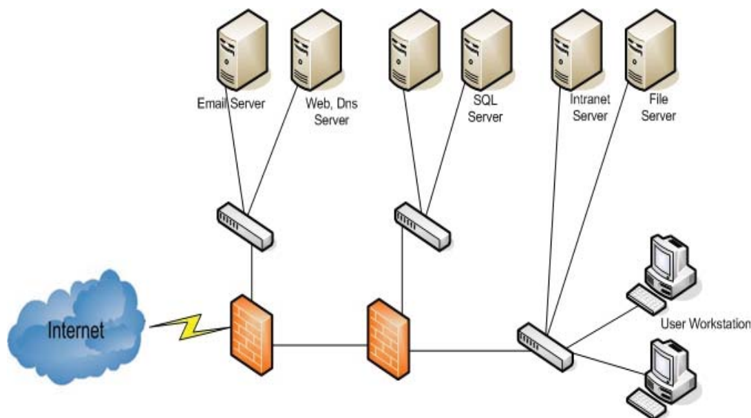
Fig. 1 Defense-in-Depth principle [6]
