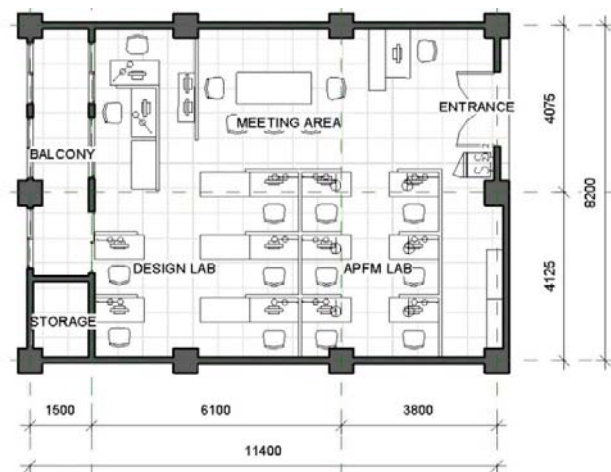
Fig. 2 RB906 Layout Plan
