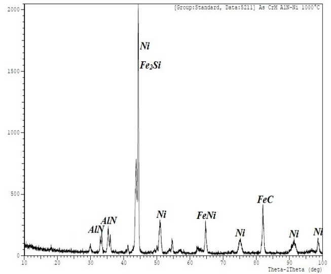
Fig. 7 X-ray diffraction patterns of the (80% Astaloy Cr-M+10% AlN) 10% Ni sintered at 1000°C
