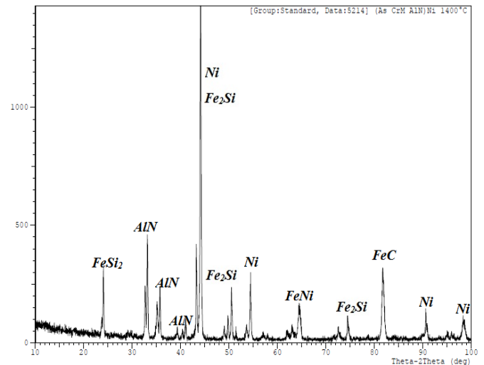
Fig. 8 X-ray diffraction patterns of the (80% Astaloy Cr-M+10% AlN) 10% Ni sintered at 1400°C
