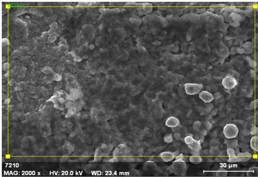
Fig. 1 SEM micrographs of as-received Ni Plated 80% Astaloy Cr-M + 10% AlN Mag.2kX 1400 °C
