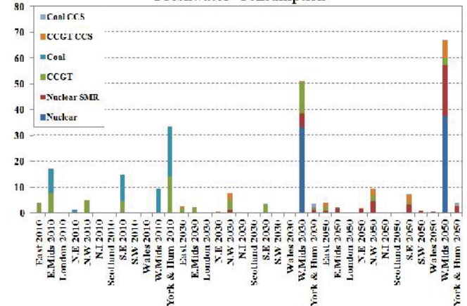
Fig. 14 Freshwater Consumption by Generation Technology ( \times 10^3 ML/Annum)
