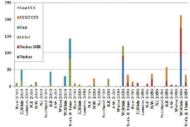
Fig. 13 Freshwater Abstraction by Generation Technology ( \times 10^3 ML/Annum)
