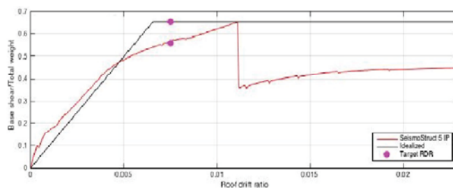
Fig. 16 NSA in SeismoStruct with 5 integration points
