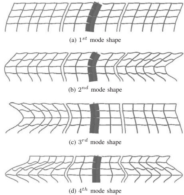
Fig. 4 First four natural mode shapes of the model according to SeismoStruct
