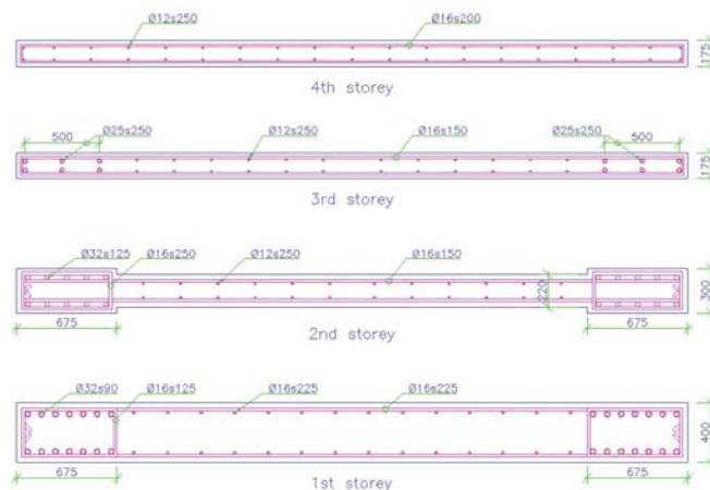
Fig. 2 Wall sections
