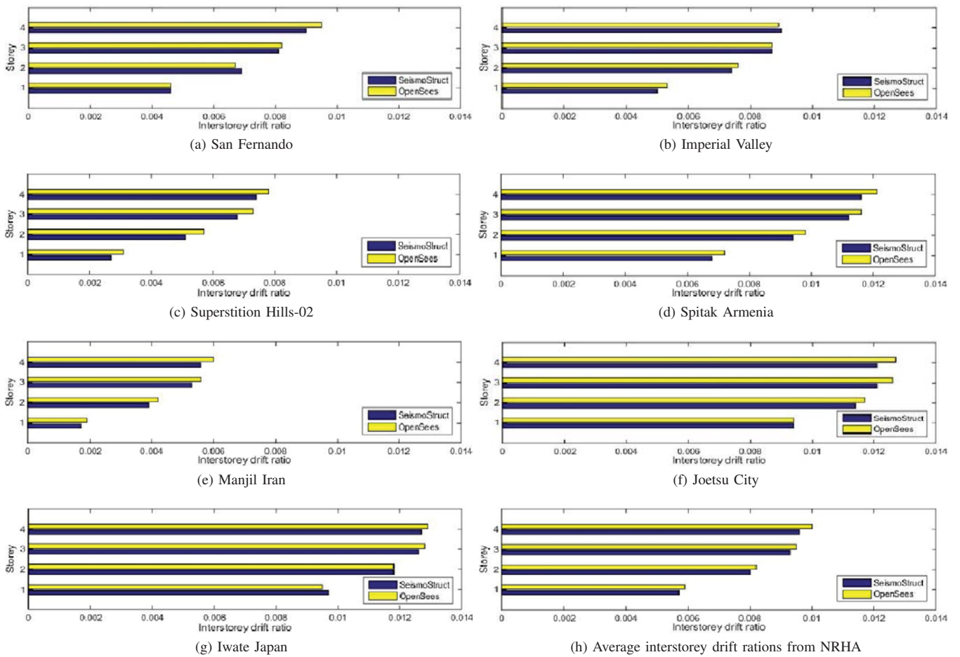
Fig. 9 Maximum interstorey drift ratios from the nonlinear time history analyses
