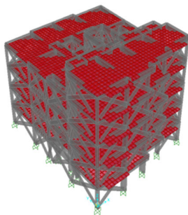
Model III: Layered shell infill model
