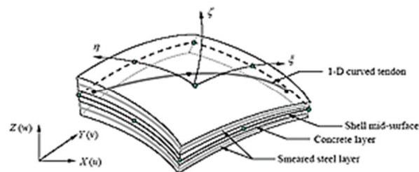
Fig. 2 Multi-layer shell element
