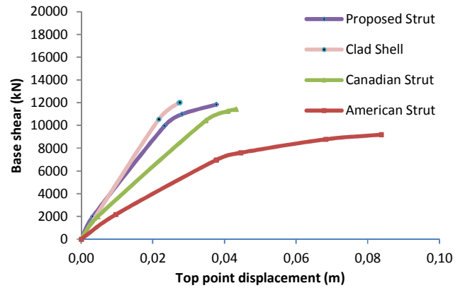
(a) Static nonlinear analysis X-X
