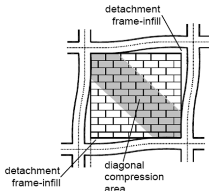
Fig. 4 Strut model analogy of in-filled frames
