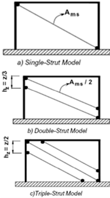
Fig. 3 Modified strut models adapted from [20]
