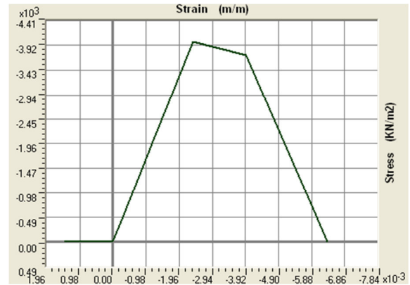
(c) Stress-strain curve for clad brick
