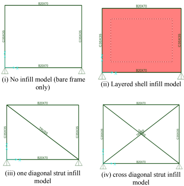
Fig. 8 Four different modeling for the comparative example
