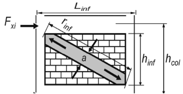
Fig. 5 Compression strut analogy—concentric Struts, ASCE/SEI 41-06 B. NBCC 2005
