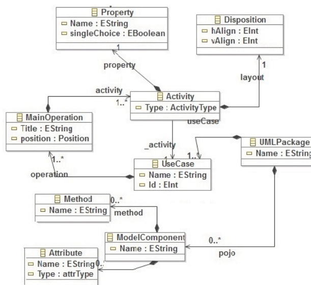
Fig. 4 Proposed GUI PIM meta model for RIA
