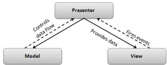
Fig. 2 The MVP design pattern
