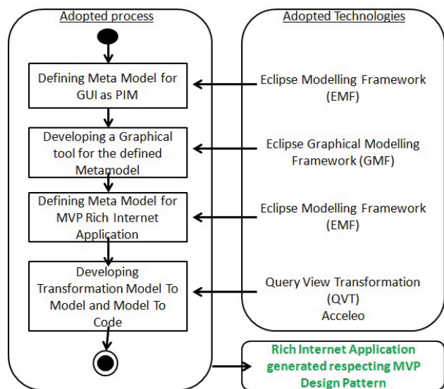
Fig. 3 Process and technologies adopted to define our model-driven approach
