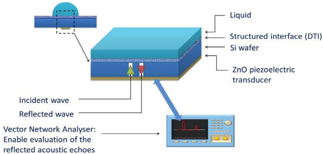
Fig. 3 High-frequency acoustic reflectometry principle
