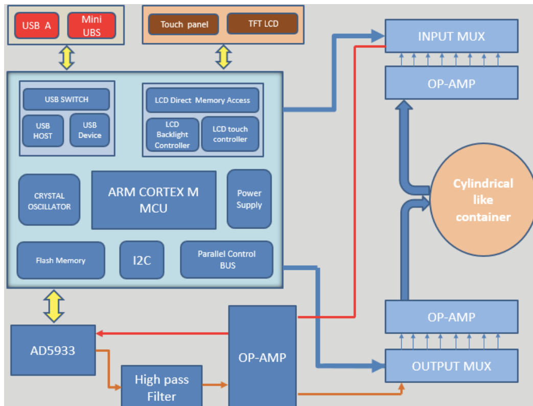
Fig. 1 Device hardware block diagram
