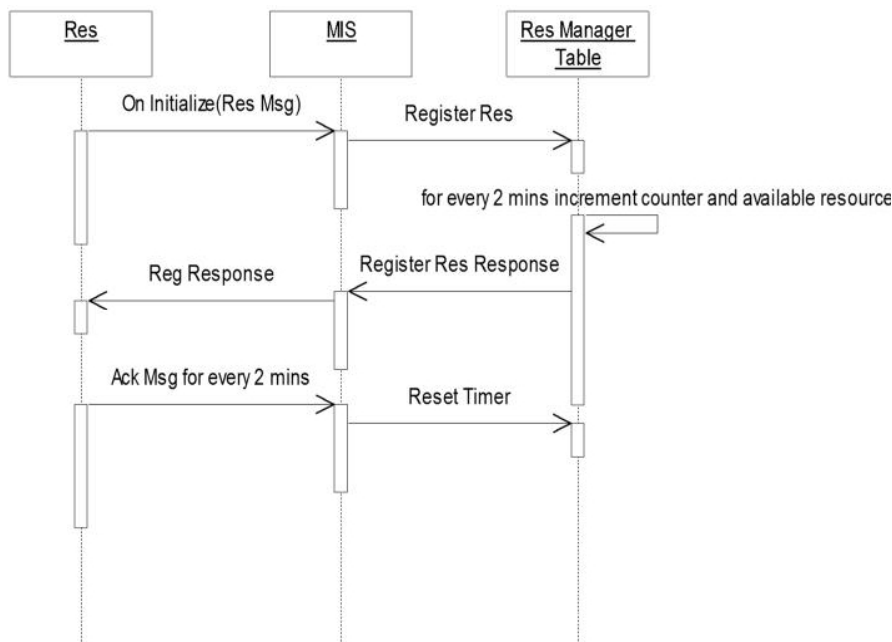
Fig. 2 Sequence Diagram of LSAP
