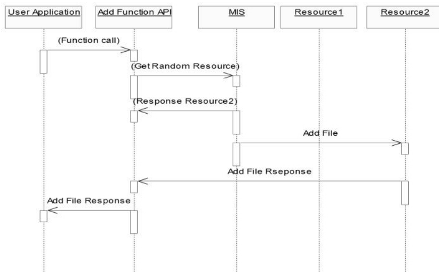
Fig. 3 Sequence diagram of add-file response
