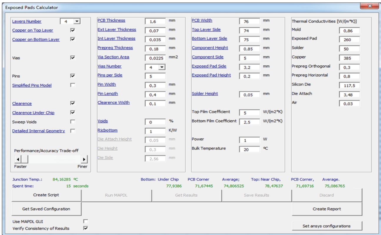
Fig. 8 User-friendly interface in Visual Basic for Applications
