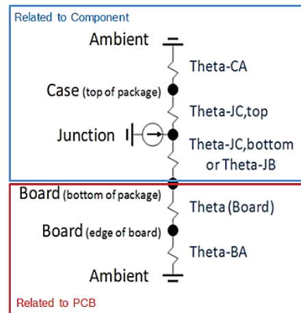
Fig. 3 Thermal resistance equivalent model (2-R)
