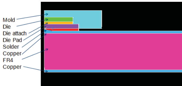
Fig. 5 Model defined in Mechanical APDL script
