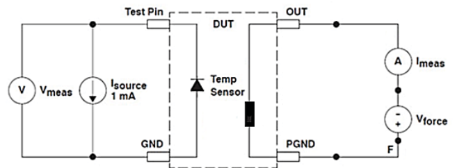
Fig. 10 Schematic diagram for T_j measurements
