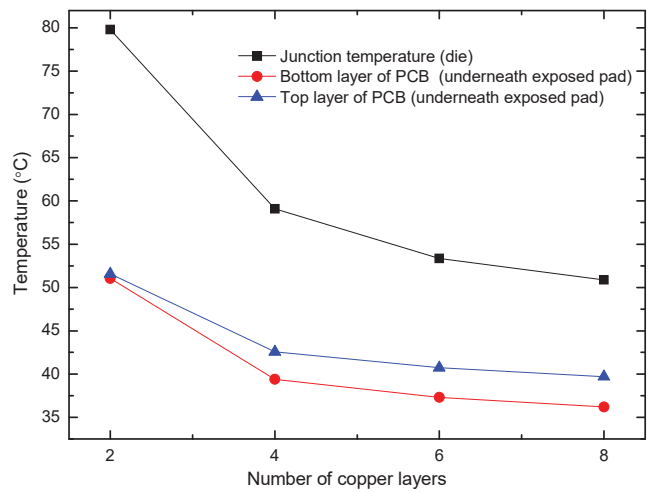
Fig. 16 temperature on different locations as a function of PCB copper layers' number
