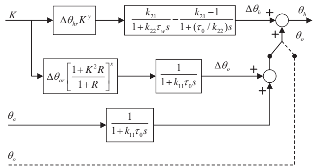
Fig. 2 Block diagram representation of the differential equations
