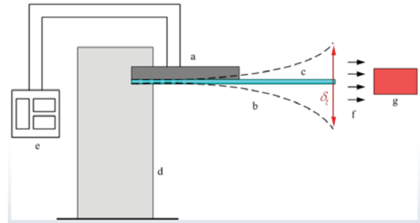
Fig. 1 Piezoelectric cooling fan (a: piezoelectric actuator; b: piezoelectric cooling fan; c: blade; d: fixture; e: electric power; f: air flow; g: hot electronic device; \delta_t : total tip displacement)
