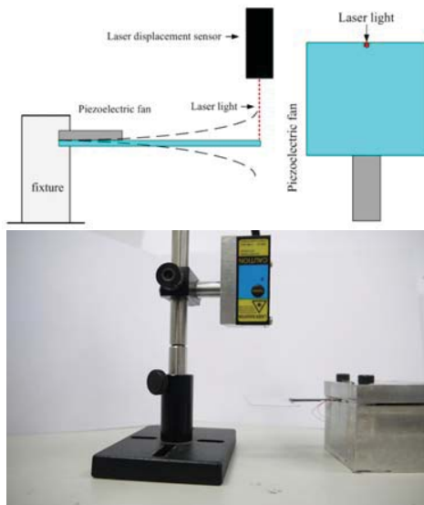
Fig. 7 Experimental equipment for vibration
