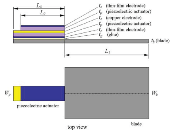
Fig. 2 Geometry property of piezoelectric cooling fan
