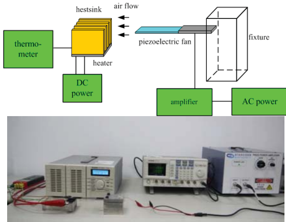
Fig. 6 Experimental equipment for cooling performance
