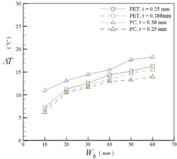
Fig. 12 \Delta T versus W_b . ( L_l = 60 mm)
