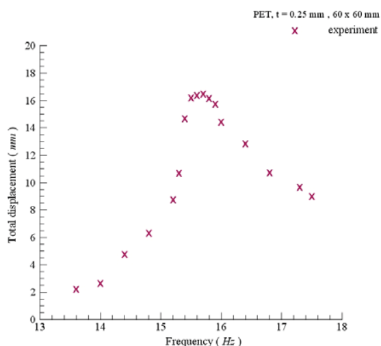
Fig. 10 Total displacement \delta obtained from experiments (first mode; L_l=60 mm, W_b=60 mm, t_b=0.25 mm; PET; V_{amp}=100 V)
