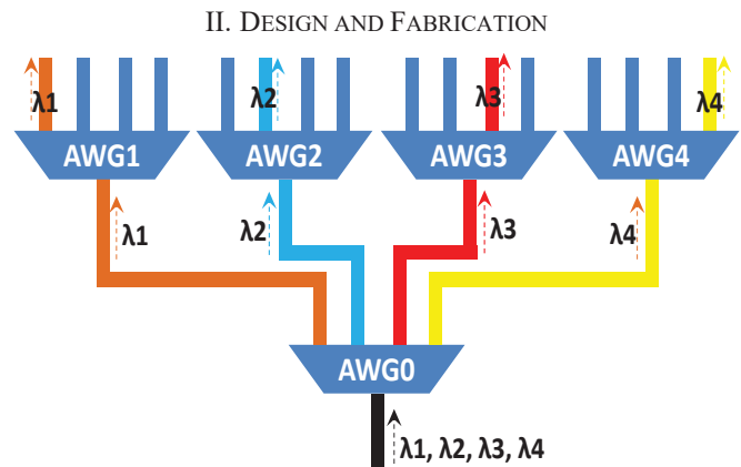
Fig. 1 Schematic of 1 \times 4 cascaded silicon photonic AWG
